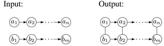
Figure 6: The association transduction
